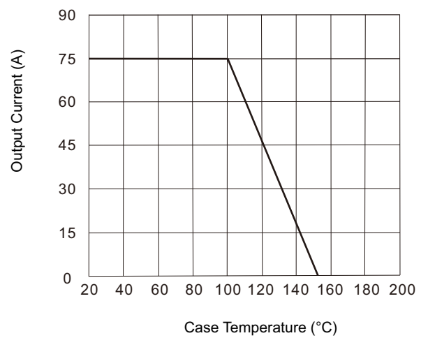
Fig.4 Case temperature vs output current
