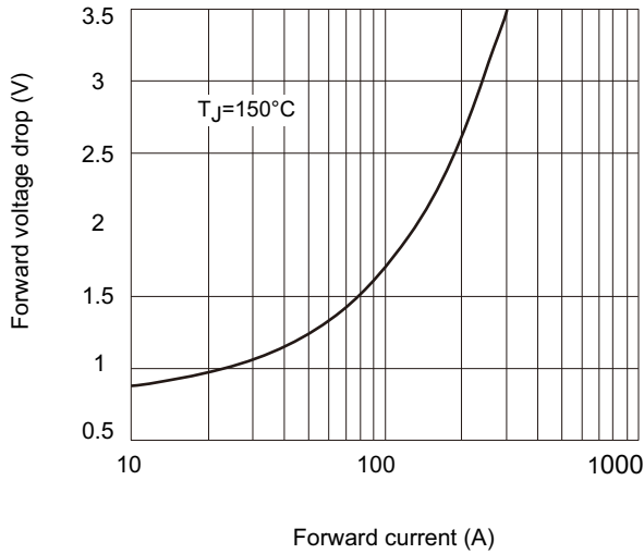
Fig.1 Forward characteristic
