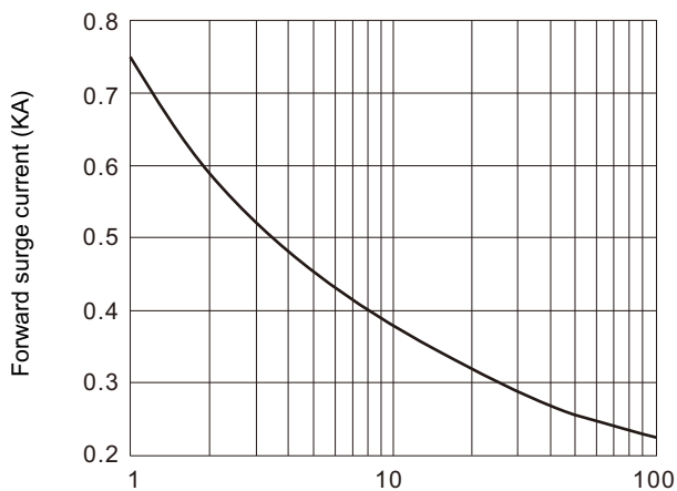
Fig.5 Forward surge current vs. cycle
