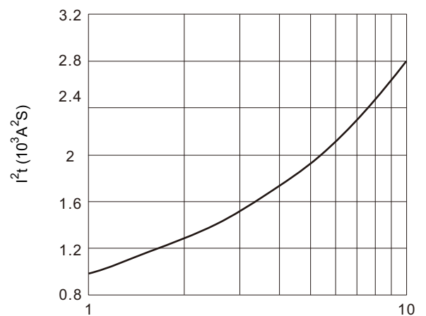
Fig.6 I^2t characteristic
