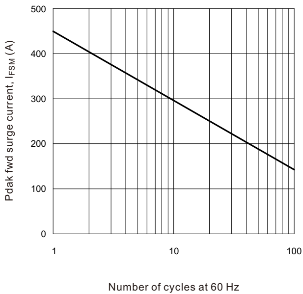
Fig.3 Max non-repetitive peak surge current
