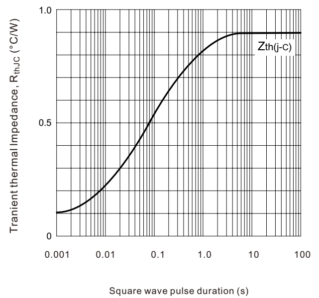
Fig.4 Transient thermal impedance
