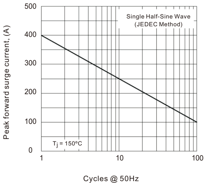
Fig.3 Maximum non-repetitive peak-forward surge current per leg
